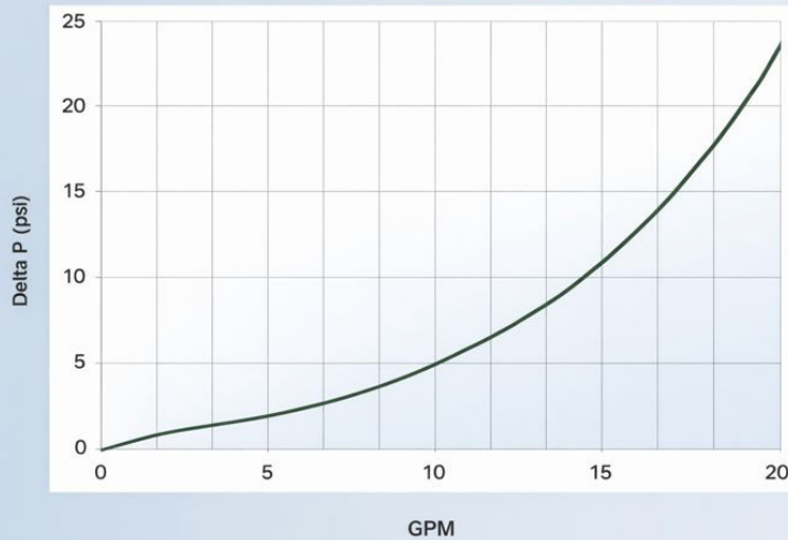
Flow Rate/Pressure Drop
