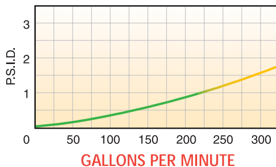
BF 850-FL PERFORMANCE CURVE*
