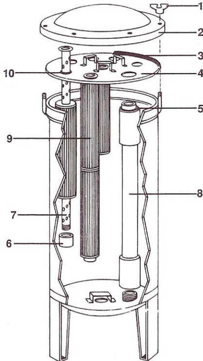
Models BF96, BF144
