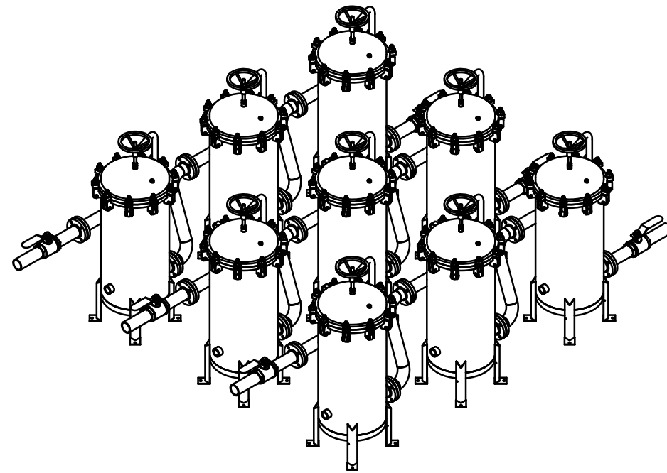
ISOMETRIC VIEW
